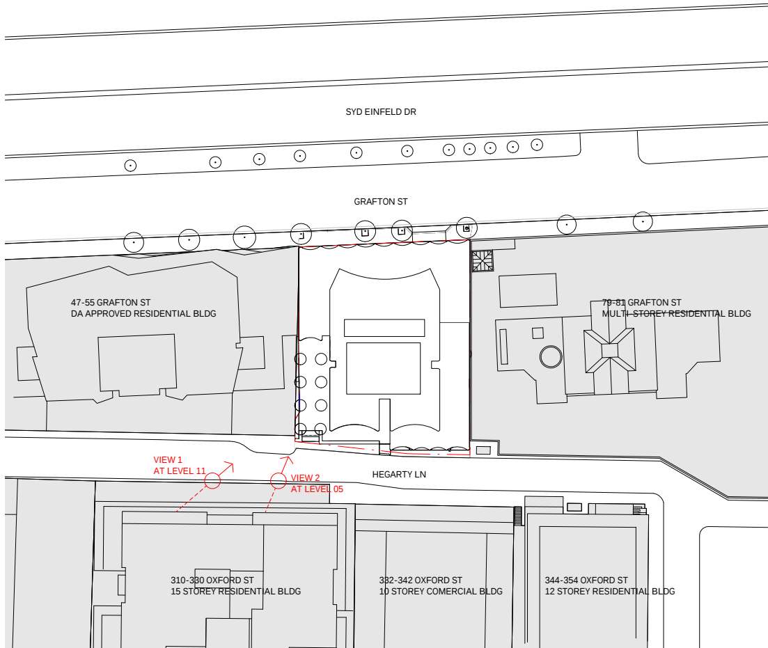
3 KEY PLAN
